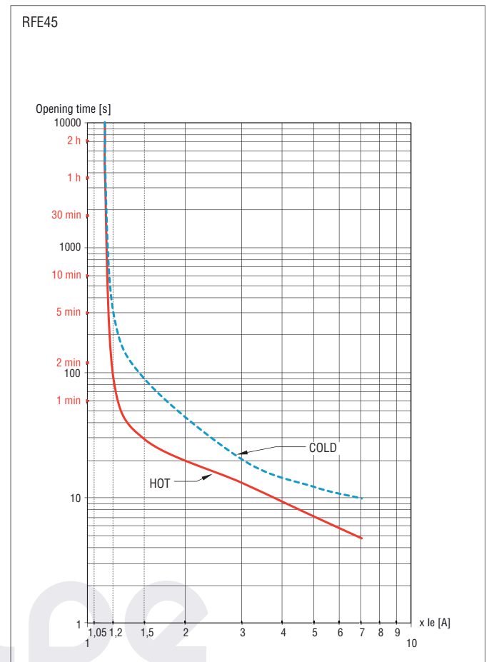
Three-phase balanced operation; class 30
