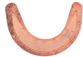
Deep Indent on Aluminum Flexible Cable
